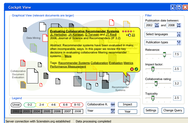
Figure 1: GUI SciPlore – clustering similar documents
